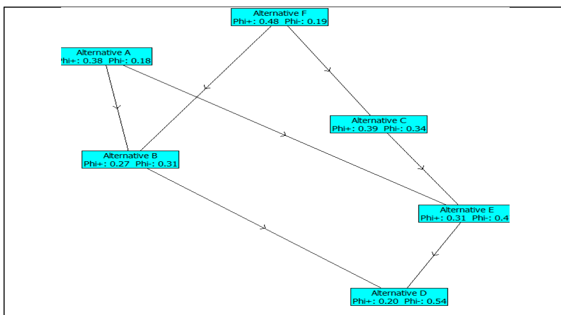
Fig. 8. Promethee network
